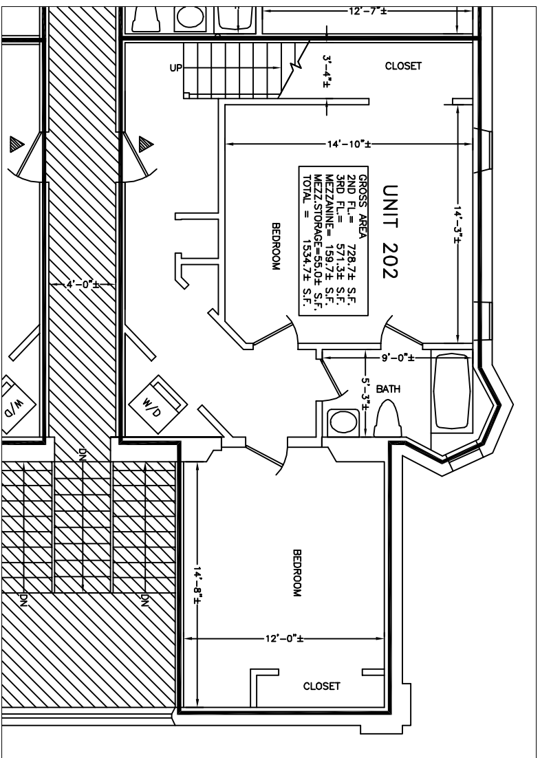
UNIT 202 SECOND FLOOR
