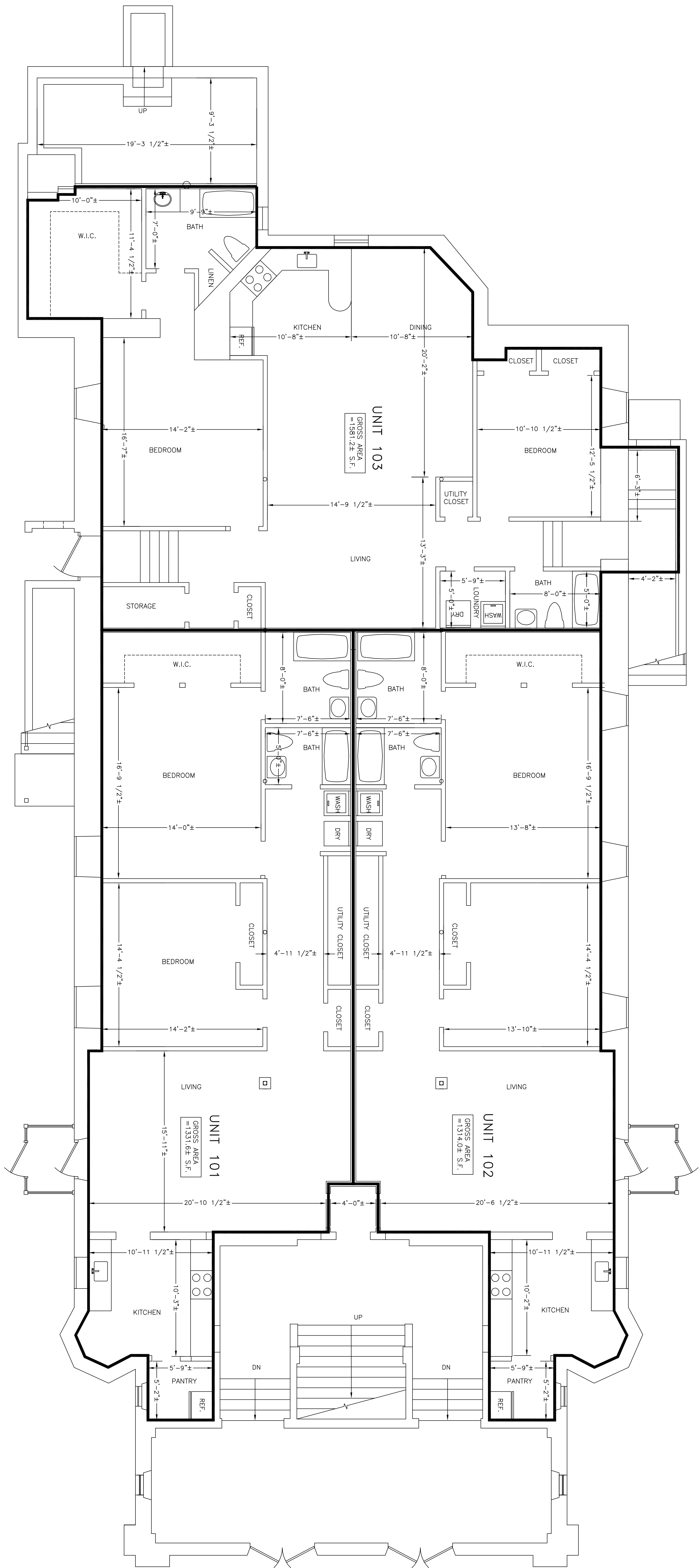
PROPOSED FIRST FLOOR PLAN
